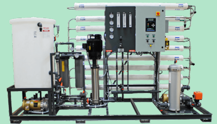
Industrial Reverse Osmosis System with Membrane Clean-In-Place & Permeate Flush System
